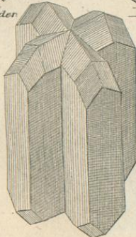
XXI. Staurolith-Zwilling.
