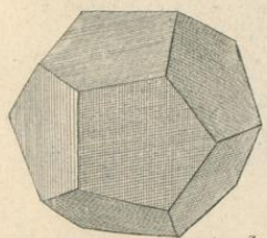
XIX. Pentagon-Dodekaeder.
