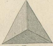
XVII. Tetraeder.
