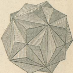
XXII. Eisenarsen-Zwilling.
