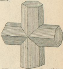
XX. Hexaeder-Zwilling
